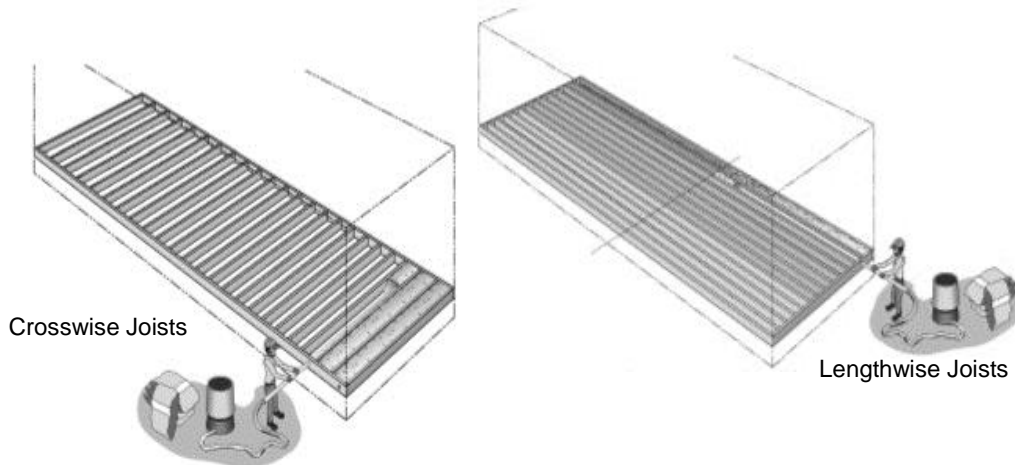
Insulating through the rim joist: Mobile homes have either lengthwise or crosswise joists.
